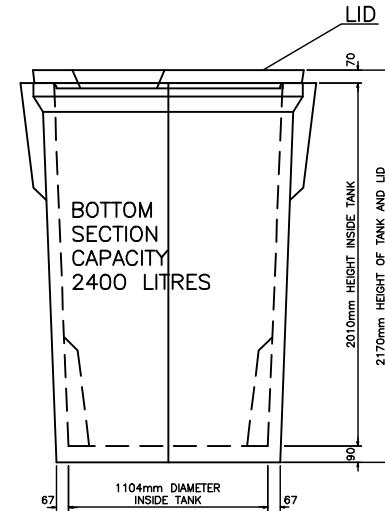
ELEVATION OF BOTTOM SECTION OF TANK WITH LID
