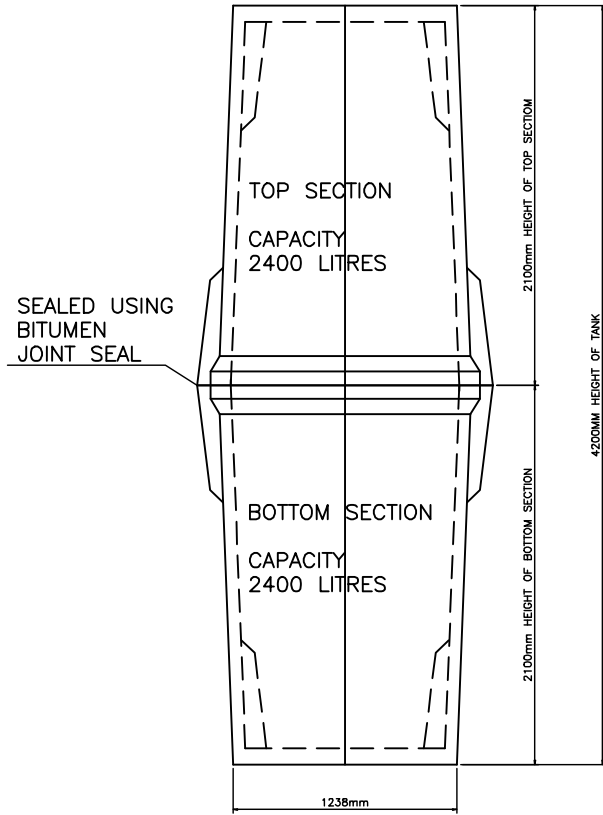
ELEVATION OF BOTH SECTIONS OF TANK
