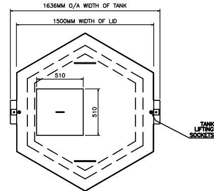
PLAN OF LID FOR BOTTOM SECTION OF TANK
